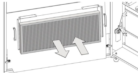
Servicetür filter
