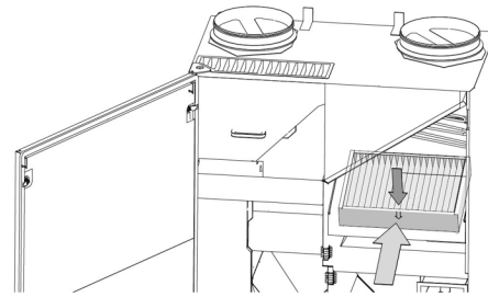
Inner filter
