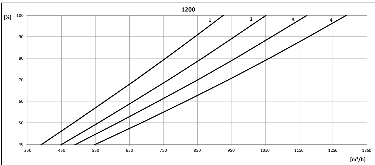
1: Ecke, 30 dB(A); 2: Center, 30 dB(A); 3: Ecke, 35 dB(A); 4: Center, 35 dB(A)
